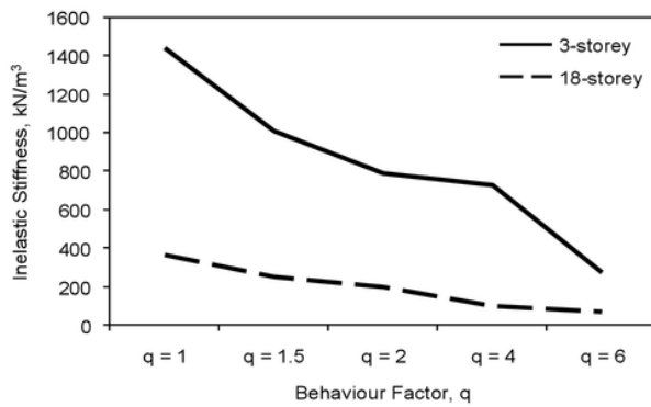
Fig. 5. Inelastic stiffness.
