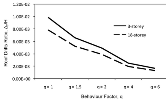
Fig. 4. Roof drifts ratio.
