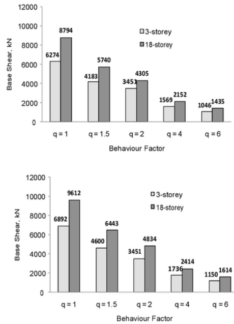
Fig. 6. Lateral strength: Base shear at yield (top) and maximum base shear (bottom).
