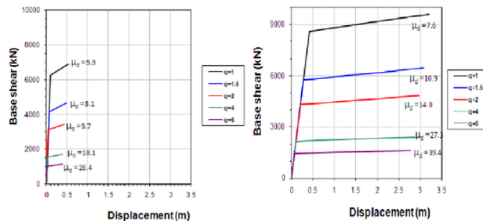
Fig. 3. Capacity curve for 3-storey (top) and 18-storey models (bottom).
